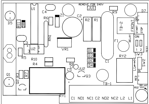
Figure 2. Board Layout
